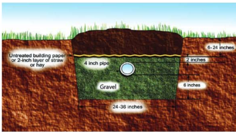
Figure 3: Trench with pipe lateral.
