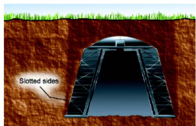
Figure 4: Gravelless chamber for effluent treatment.
