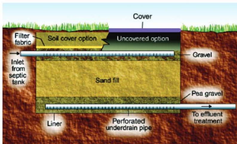
Figure 6: Sand filter.
