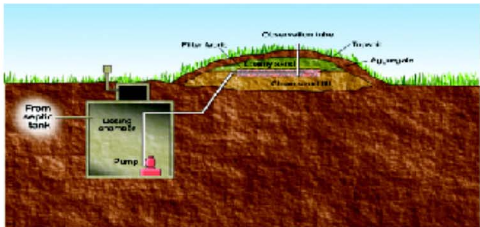
Figure 5: Mound system.
