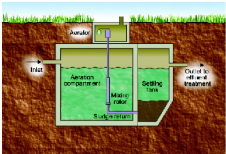
Figure 7: Aerobic treatment unit.
